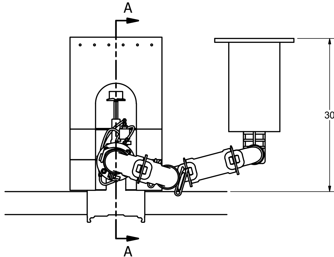
④ CONTROL VALVE, PIPING, AND TURF SPRINKLER DETAIL UNDER SYNTETIC FIELD NO SCALE
